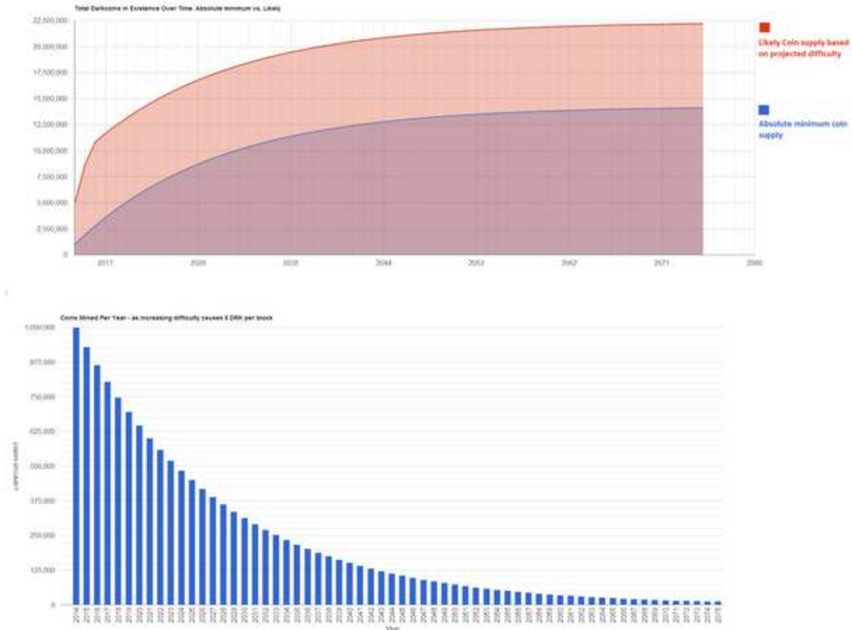
Figure 6: Mining Reward Schedule
