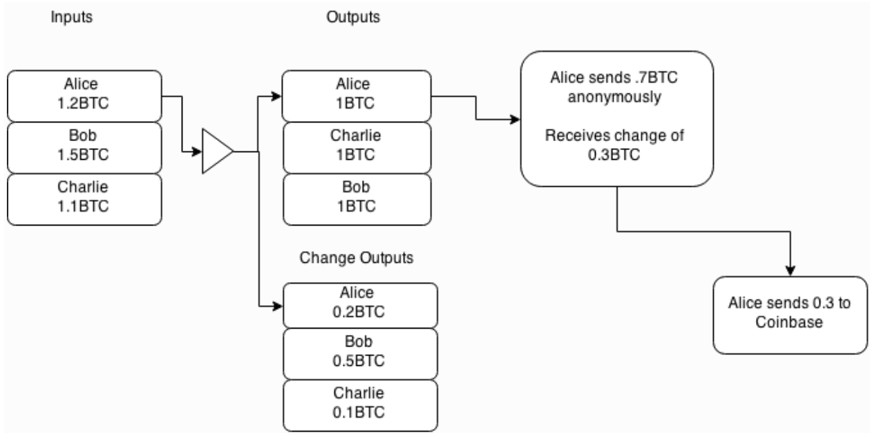
Figure 3: Forward Change Linking
